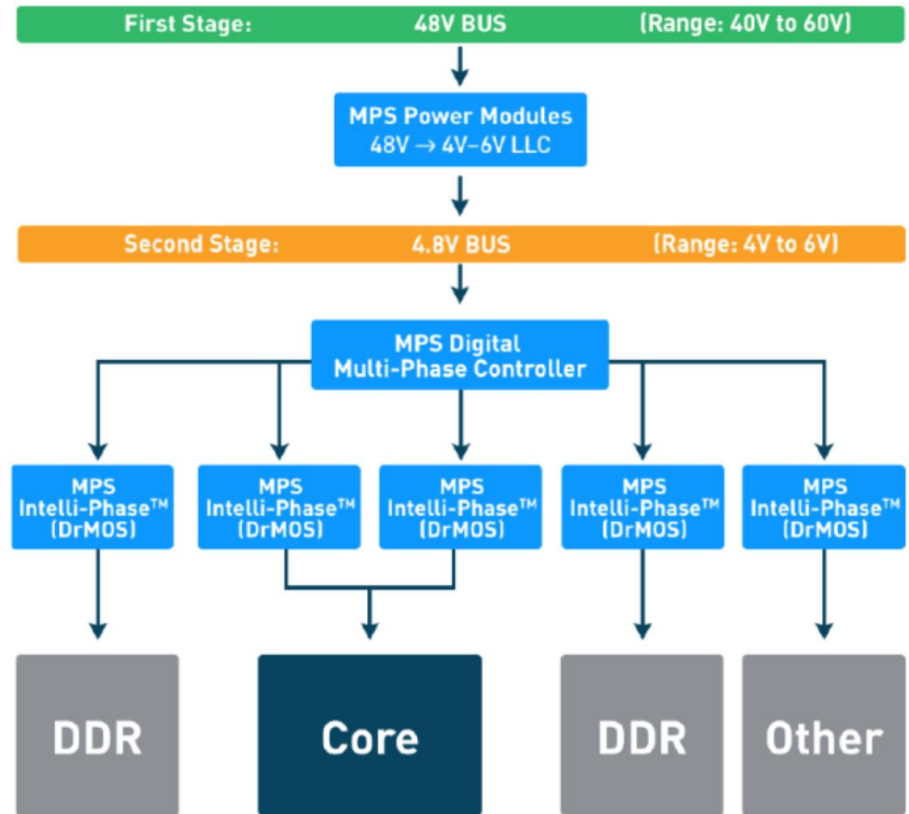
Figure 2: 48V Power Structure – MPS 4V to 6V System
